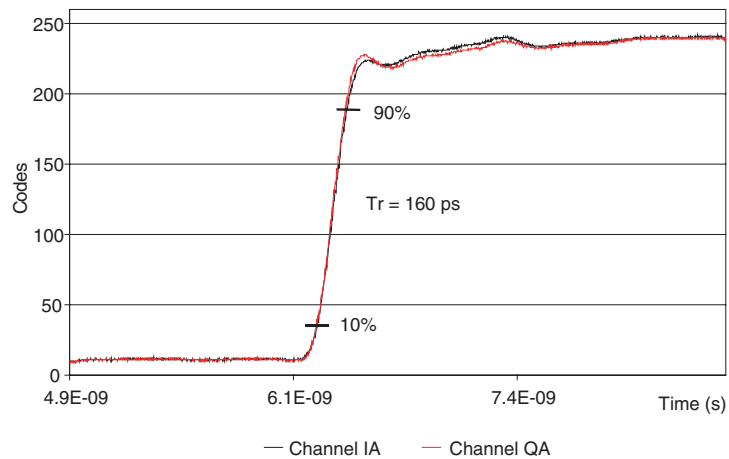
Figure 6-6. Step Response (Zoom)
