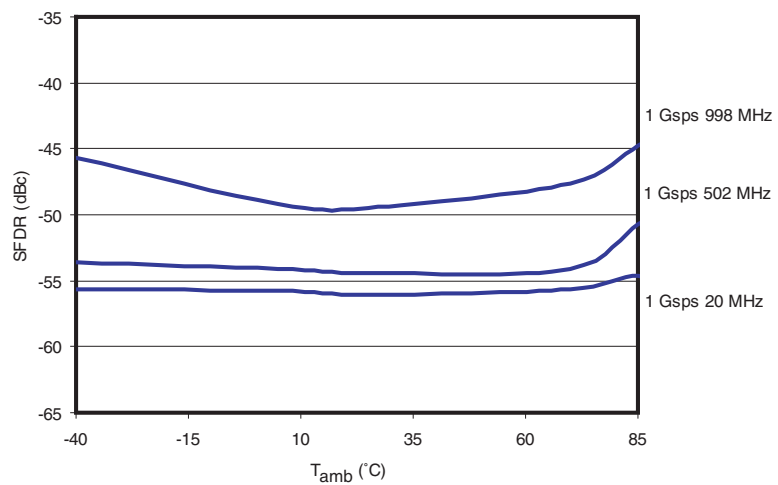
Figure 6-27. SFDR Versus Ambient Temperature ( F_s = 1 Gsps, 1:2 DMUX, F_s/4 DR Type, ISA = -50 ps)
