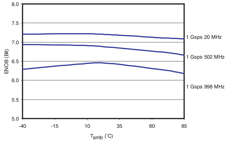
Figure 6-26. ENOB Versus Ambient Temperature ( F_s = 1 Gsps, 1:2 DMUX, F_s/4 DR Type, ISA = -50 ps)
