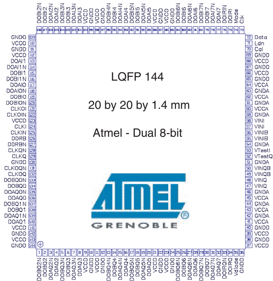
Figure 5-1. AT84AD001B Pinout (Top View)
