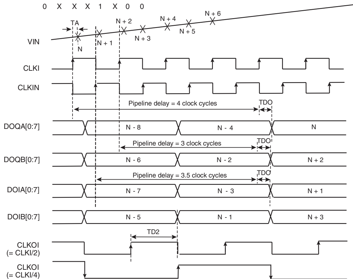
Figure 4-6. 1:2 DMUX Mode, Clock I = ADC I, Clock IN = ADC Q
