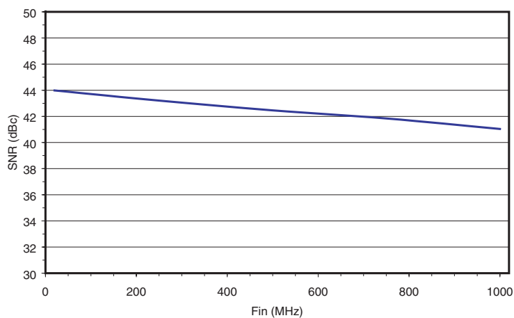
Figure 6-16. SNR Versus Input Frequency ( F_s = 1 Gsps)
