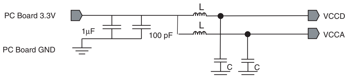
Figure 10-1. V_{CCD} and V_{CCA} Bypassing and Grounding Scheme
