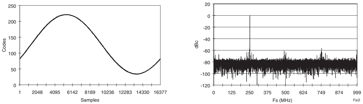
Figure 6-21. F_s = 1 Gsps and F_{in} = 250 MHz (Interleaving Mode F_{int} = 2 Gsps, F_s/4 DR Type, F_iSDA = -15 ps, ISA = -50 ps)
