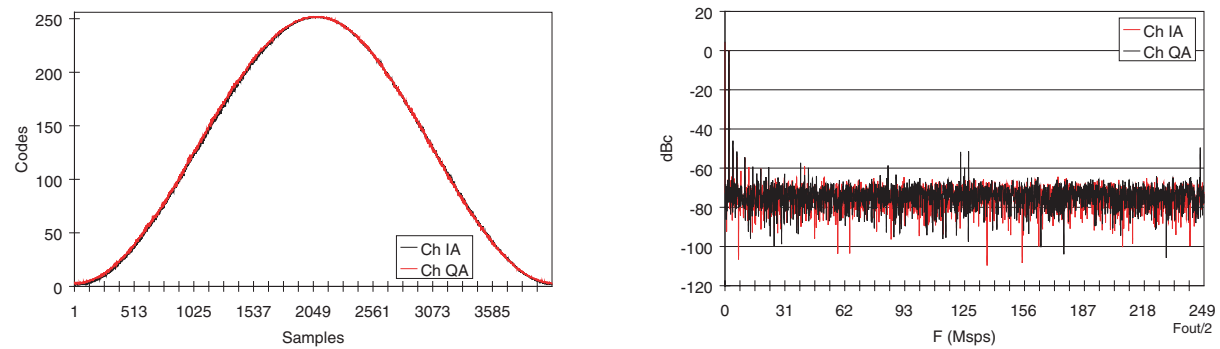
Figure 6-19. F_s = 1 Gsps and F_{in} = 1 GHz (1:2 DMUX, F_s/2 DR Type, F_iSDA = -15 ps, ISA = -50 ps)
