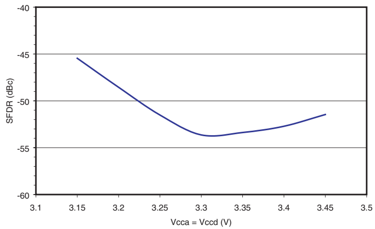
Figure 6-23. SFDR Versus V_{CCA} = V_{CCD} ( F_s = 1 Gsps, F_{in} = 500 MHz, 1:2 DMUX, F_s/4 DR Type, ISA = -50 ps)
