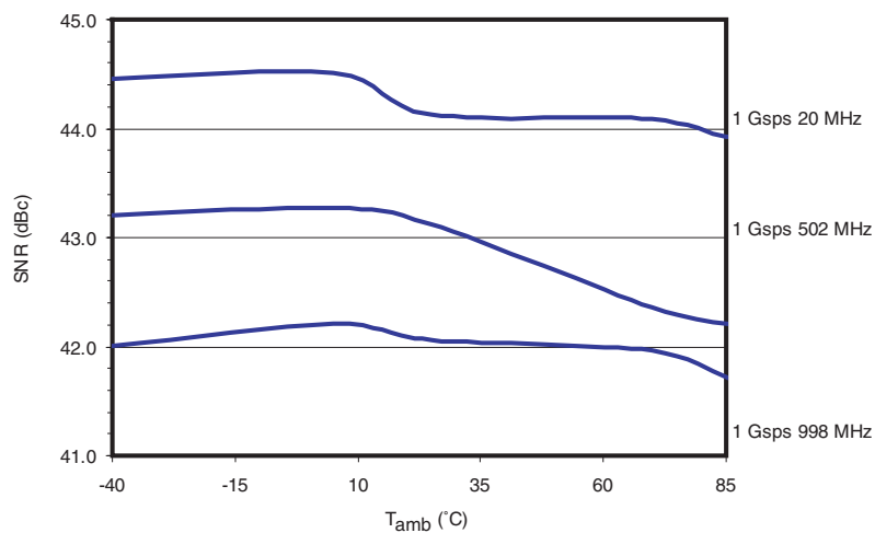
Figure 6-29. SNR Versus Ambient Temperature ( F_s = 1 Gsps, 1:2 DMUX, F_s/4 DR Type, ISA = -50 ps)
