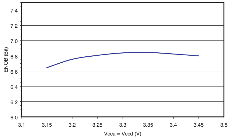
Figure 6-22. ENOB Versus V_{CCA} = V_{CCD} ( F_s = 1 Gsps, F_{in} = 500 MHz, 1:2 DMUX, F_s/4 DR Type, ISA = -50 ps)
