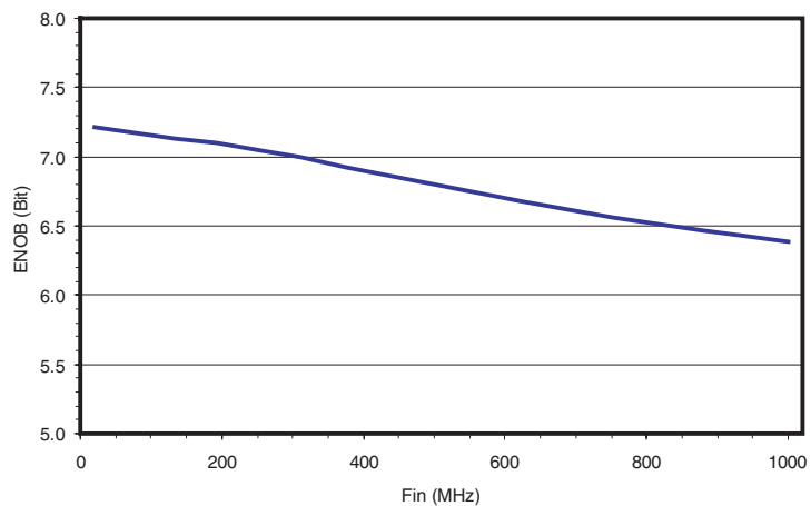
Figure 6-13. ENOB Versus Input Frequency ( F_s = 1 Gsp/s)
