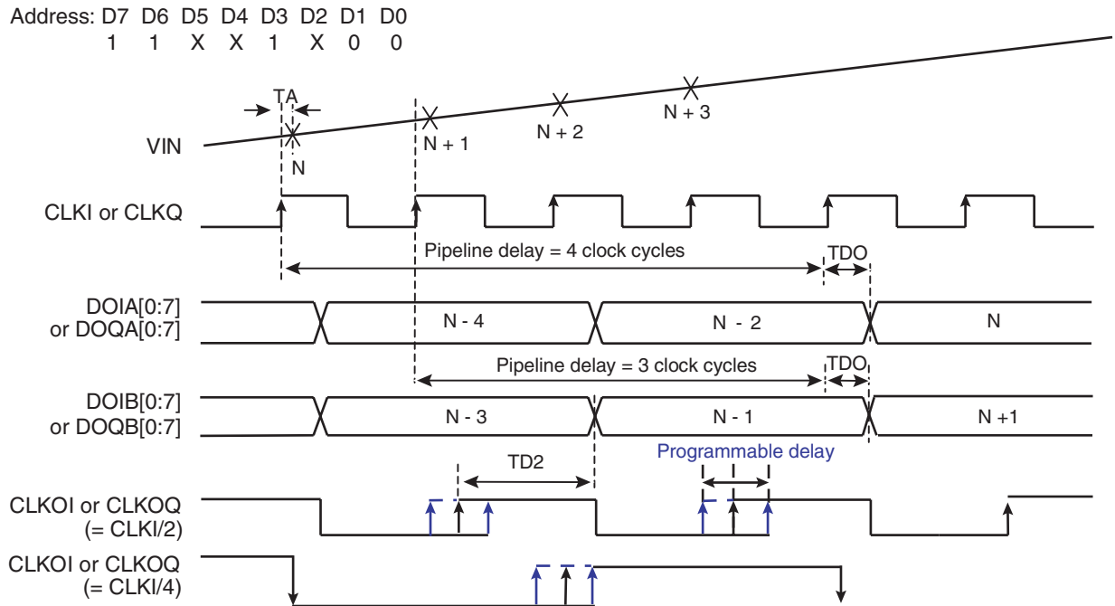
Figure 4-2. Timing Diagram, ADC I or ADC Q, 1:2 DMUX Mode, Clock I for ADC I, Clock Q for ADC Q
