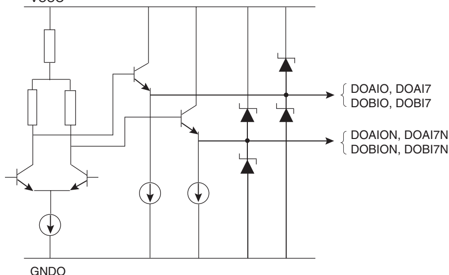
Figure 8-4. Data Output Buffer Model VCCO
