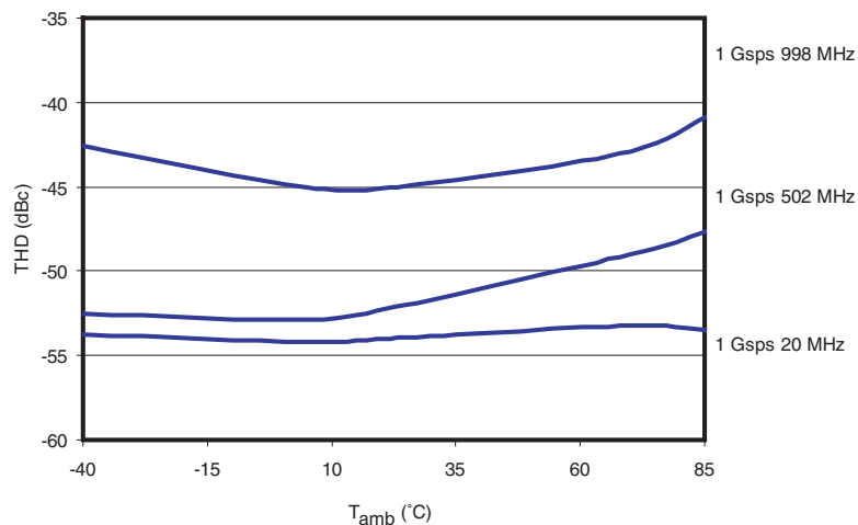
Figure 6-28. THD Versus Ambient Temperature ( F_s = 1 Gsps, 1:2 DMUX, F_s/4 DR Type, ISA = -50 ps)
