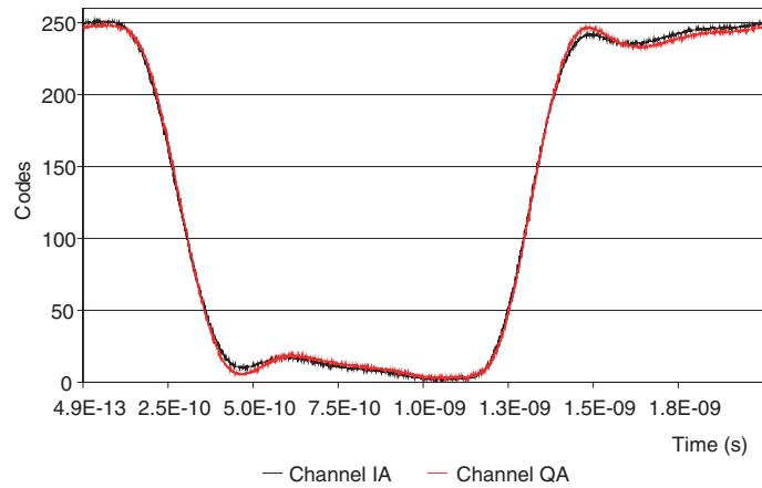
Figure 6-7. Step Response
