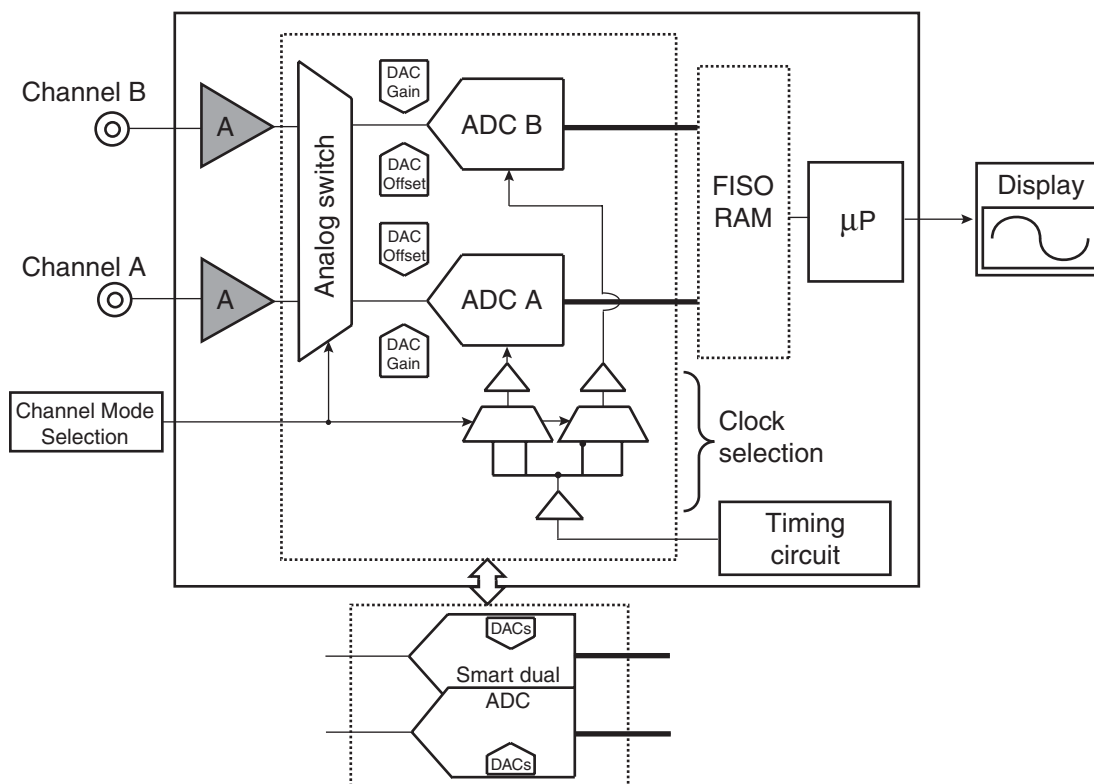
Figure 3-2. Dual Channel Digital Oscilloscope Application
