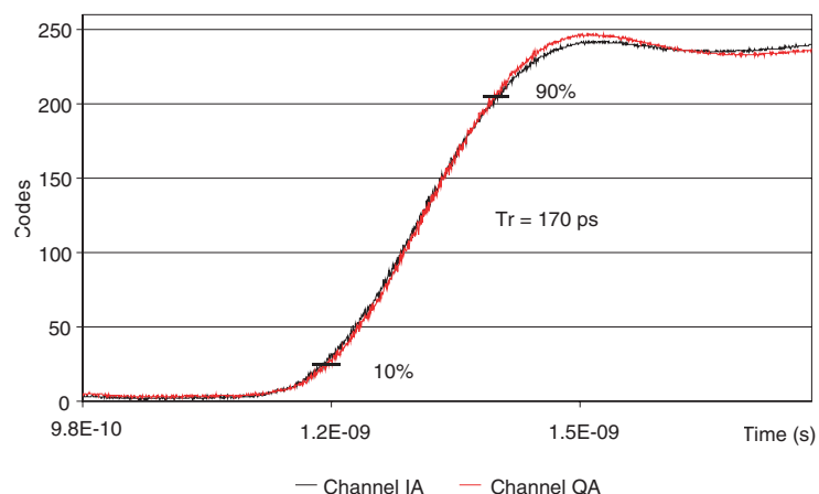
Figure 6-8. Step Response (Zoom)
