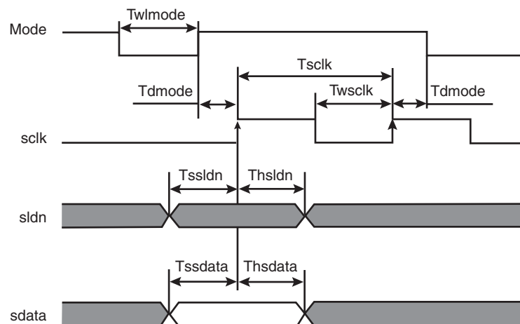
Figure 7-2. Timing Definition
