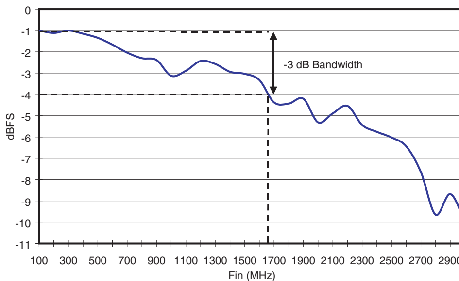
Figure 6-1. Full Power Input Bandwidth
