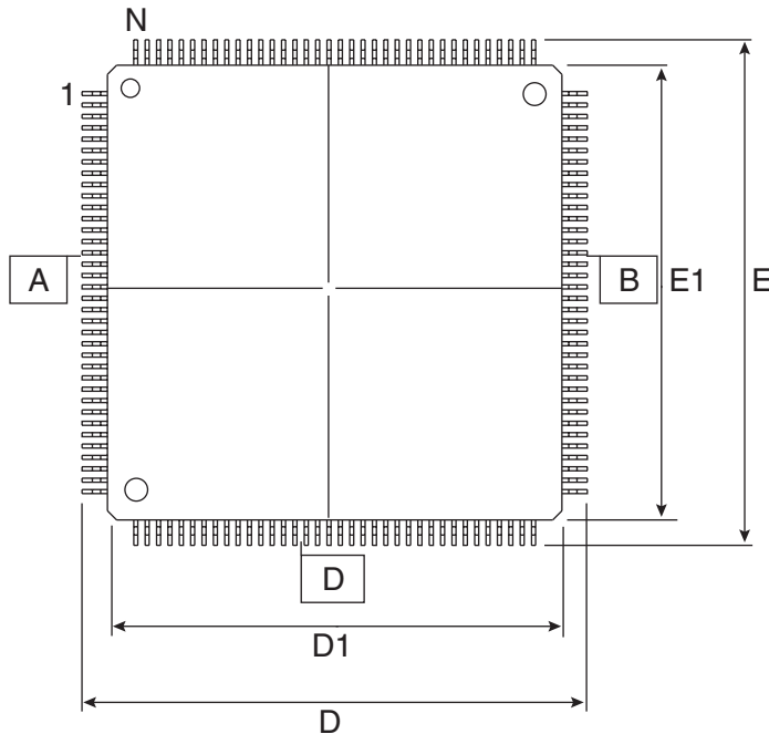
Figure 13-1. Type of Package
