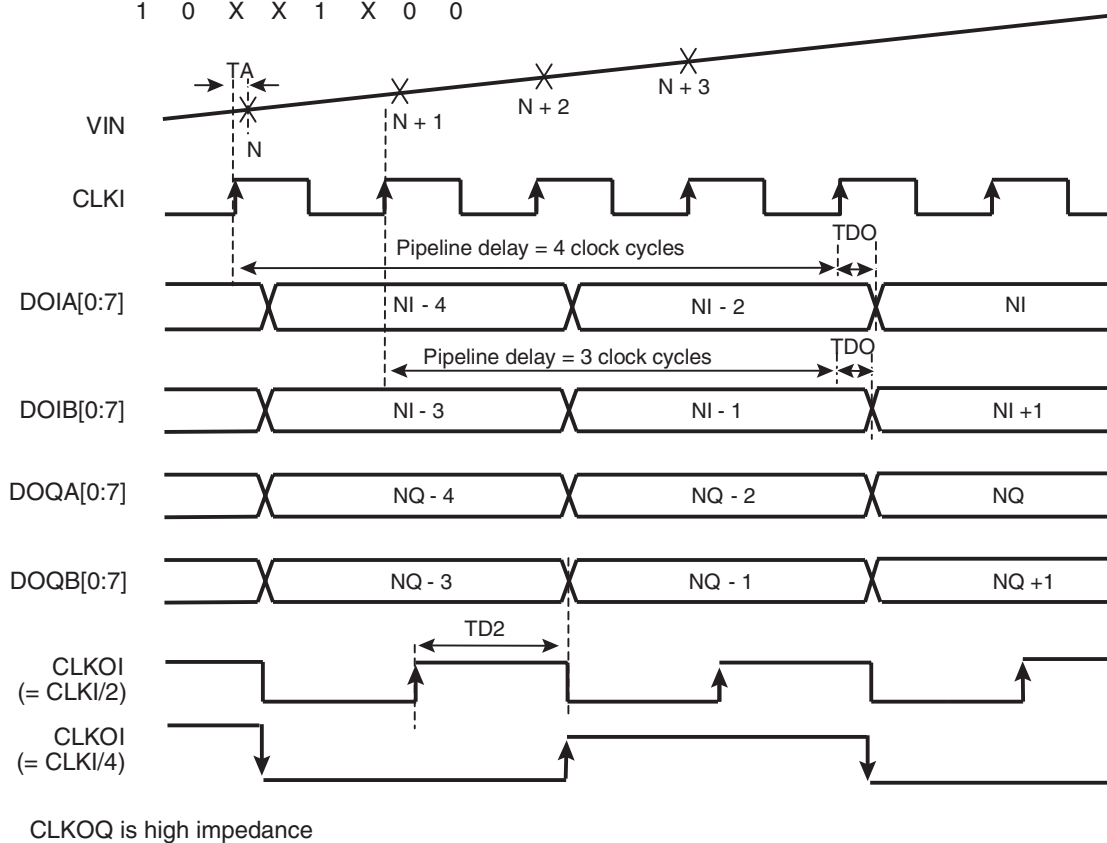
Figure 4-4. 1:2 DMUX Mode, Clock I = ADC I, Clock I = ADC Q
