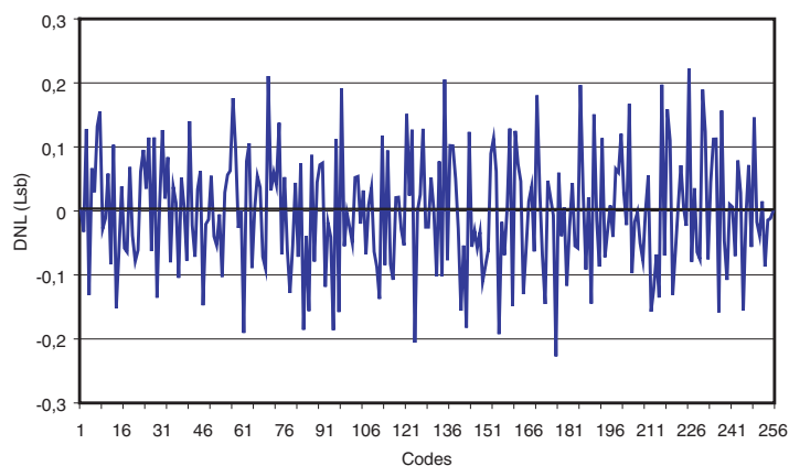
Figure 6-4. Typical DNL ( F_s = 50 Msps, F_{in} = 1 MHz, Saturated Input)
