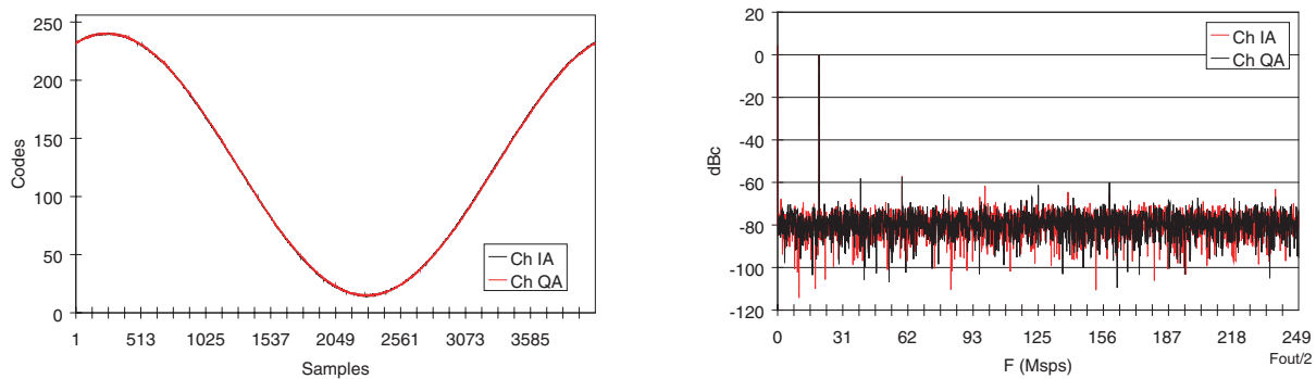
Figure 6-18. F_s = 1 Gsps and F_{in} = 500 MHz (1:2 DMUX, F_s/2 DR Type, F_iSDA = -15 ps, ISA = -50 ps)
