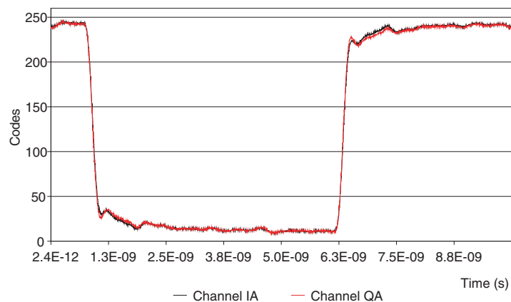
Figure 6-5. Step Response
