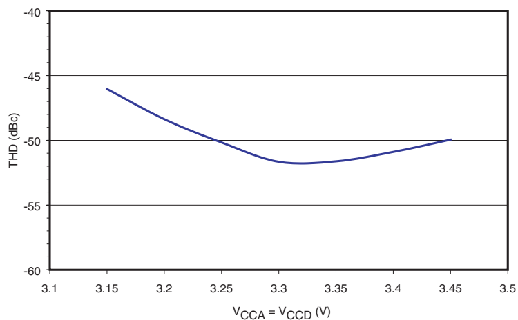
Figure 6-24. THD Versus V_{CCA} = V_{CCD} ( F_s = 1 Gsps, F_{in} = 500 MHz, 1:2 DMUX, F_s/4 DR Type, ISA = -50 ps)
