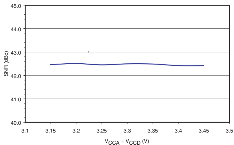
Figure 6-25. SNR Versus V_{CCA} = V_{CCD} ( F_s = 1 Gsps, F_{in} = 500 MHz, 1:2 DMUX, F_s/4 DR Type, ISA = -50 ps)
