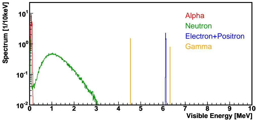
Figure 6.41: Visible Energy Spectra of ^{13}\text{C}(\alpha,n)^{16}\text{O} by Alpha Particles from ^{210}\text{Po}
