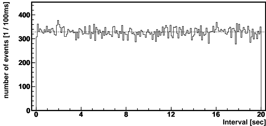
Figure 6.17: Prompt-Delayed Event Interval Distribution of Off-time Coincidence
