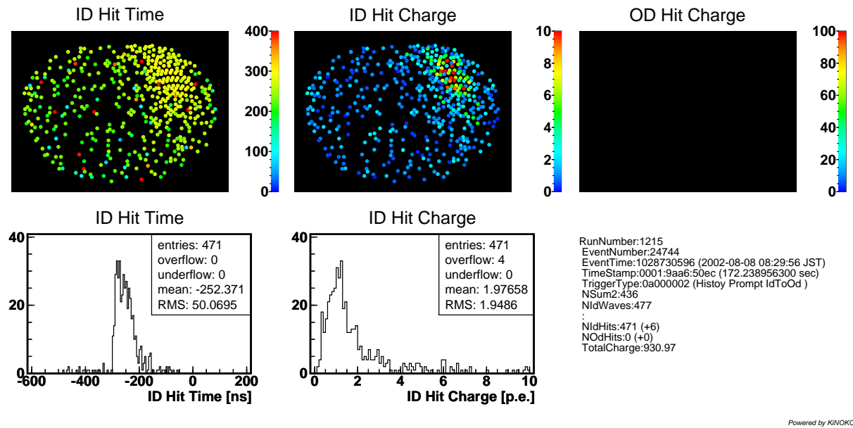
Figure 3.10: A Typical Non-Muon Event
