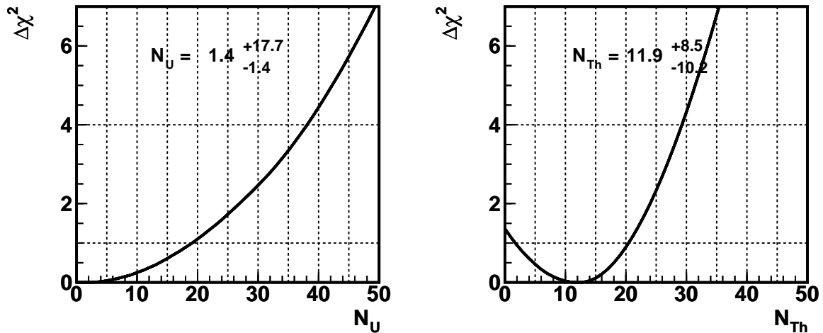
Figure 7.23: Geo-Neutrino Spectrum Rate+Shape Analysis (1-parameter estimation)
