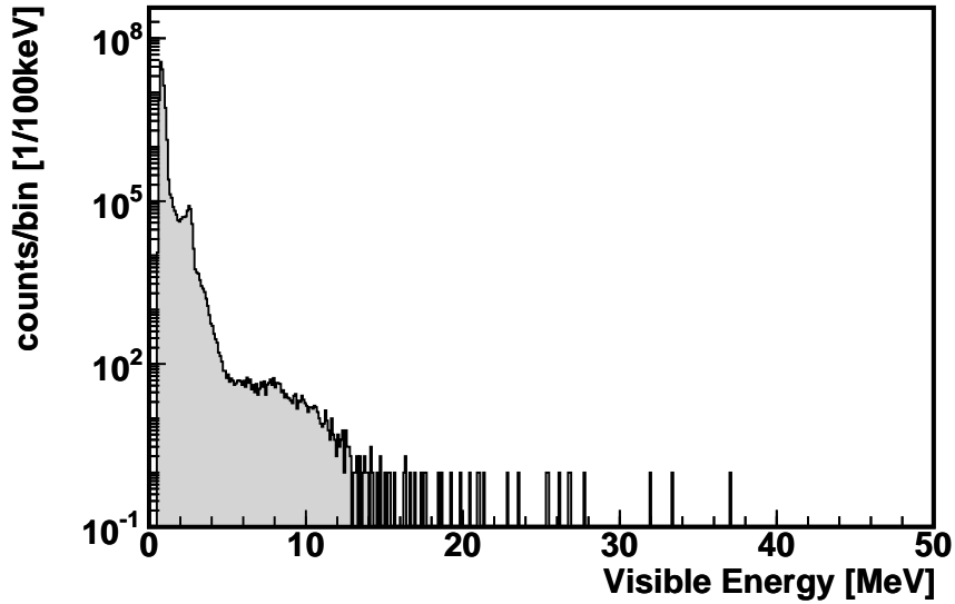
Figure 6.47: Single Event Energy Spectrum (High-Energy Region)
