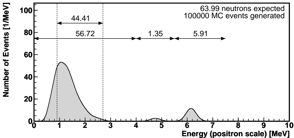
Figure 6.42: Visible Energy Spectra of ^{13}\text{C}(\alpha,n)^{16}\text{O} by Alpha Particles from ^{210}\text{Po} , with Energy Resolution
