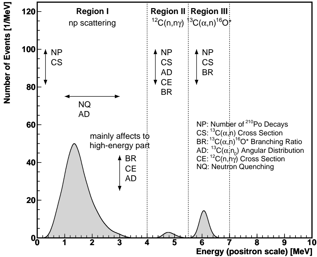
Figure 6.43: ^{13}\text{C}(\alpha,n)^{16}\text{O} Errors
