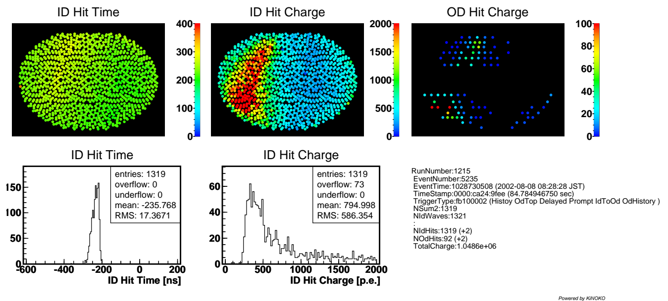
Figure 3.11: A Typical Muon Event
